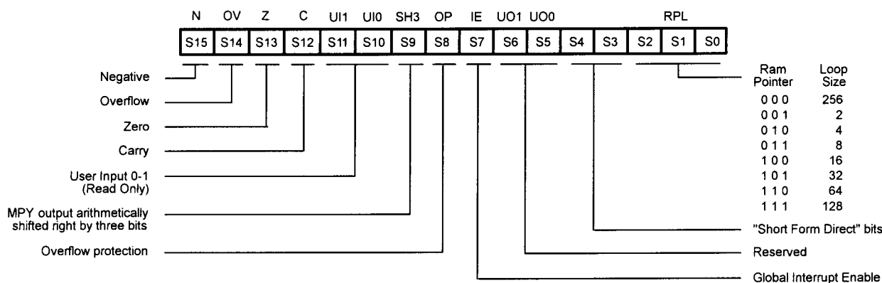
Figure 17. Status Register
