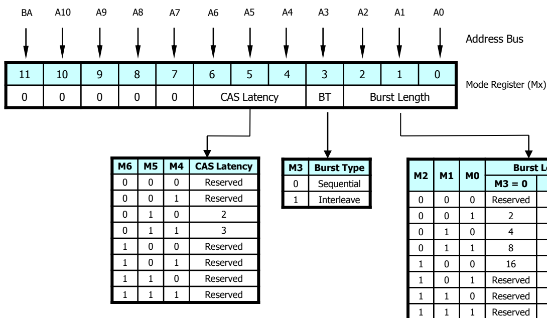
Figure4 : Mode Register Set (MRS) Definition
