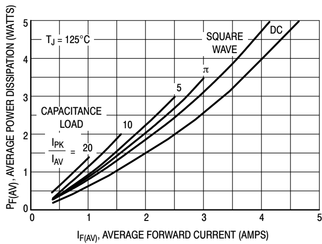
Figure 5. Power Dissipation
