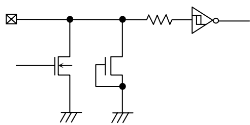
Figure 50. Input / Output Pin Circuit Diagram
