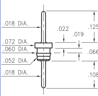
3516-0-00-XX-00-00-03-0 Press-fit in .057 mounting hole
