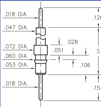
551X-0-00-XX-00-00-03-0 Press-fit in .057 mounting hole
