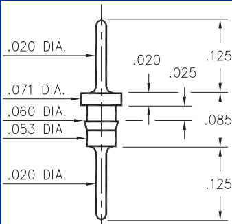
6585-0-00-XX-00-00-03-0 Press-fit in .057 mounting hole Pin material is Ph Br 544 (B2)
