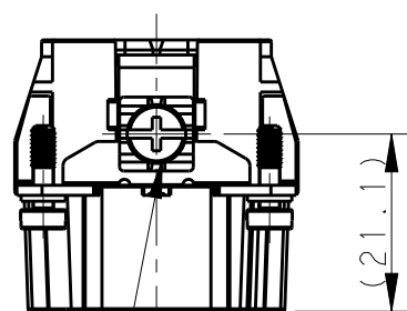
TYPE I, T2040242101-000, WITH LOGO 类型 I, T2040242101-000, 带LOGO
