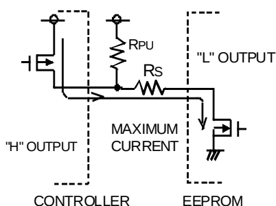
Fig.47 I/O Circuit
