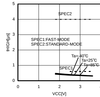
Fig.14 Data Clock High Period t_{HIGH}
