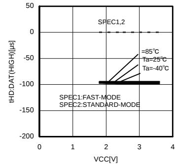
Fig.18 Data Hold Time t_{HD:DAT(HIGH)}
