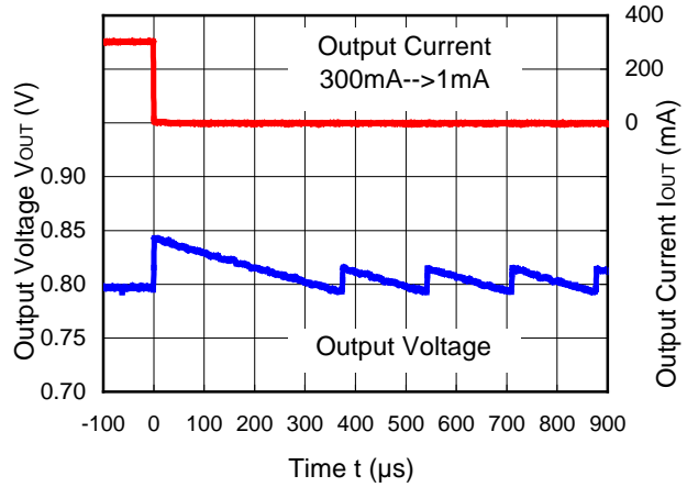
RP505K081A/B ( V_{IN}=3.6V ) MODE="H" forced PWM
