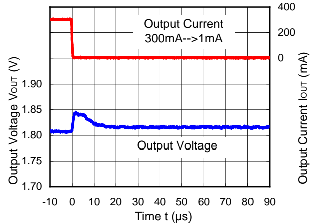
RP505K181A/B (V IN =3.6V) MODE="H" forced PWM
