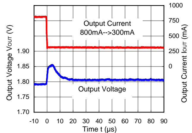
RP505K181A/B ( V_{IN}=3.6V )
