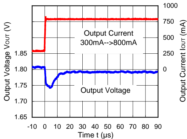
RP505K181A/B ( V_{IN}=3.6V )
