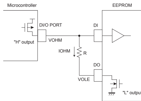
Fig. 59 Circuit at DI, DO direct connection (Microcontroller DI/O "H" output, EEPROM "L" output)
