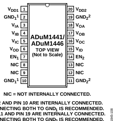
Figure 8. ADuM1441/ADuM1446 SSOP Pin Configuration
