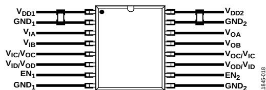
Figure 29. Recommended Printed Circuit Board Layout, QSOB
