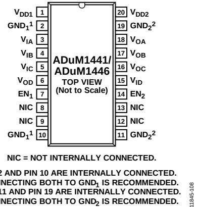
Figure 8. ADuM1441/ADuM1446 SSOP Pin Configuration
