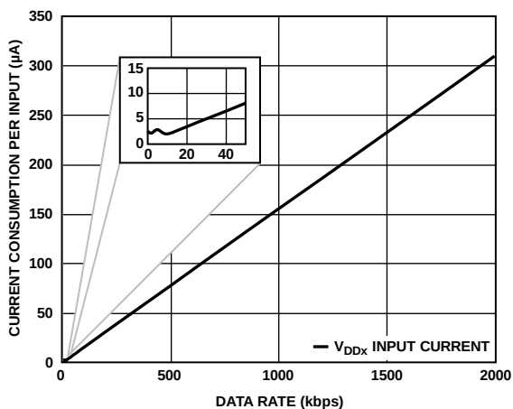
Figure 11. Current Consumption per Input vs. Data Rate for 2.5 V, \text{EN}_x = \text{Low Operation}
