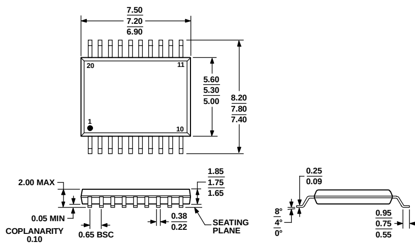
Dimensions shown in inches and (millimeters)
