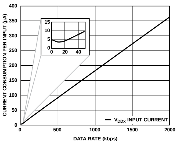
Figure 13. Current Consumption per Input vs. Data Rate for 3.3 V, \text{EN}_x = \text{Low Operation}
