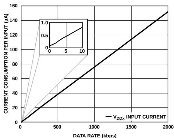
Figure 15. Current Consumption per Input vs. Data Rate for 2.5 V, \text{EN}_x = \text{High Operation}
