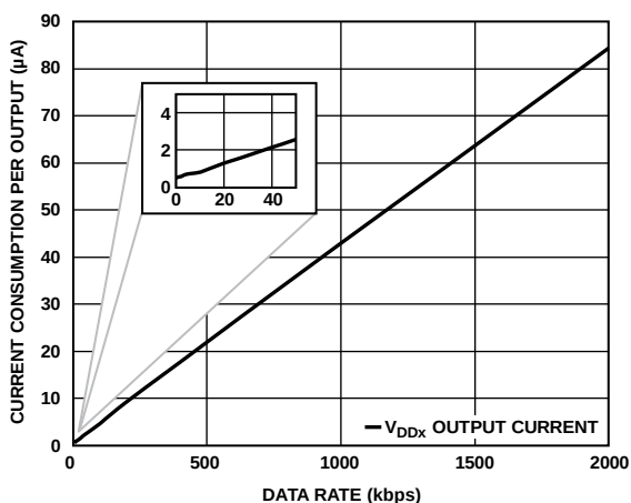
Figure 12. Current Consumption per Output vs. Data Rate for 2.5 V, \text{EN}_x = \text{Low Operation}
