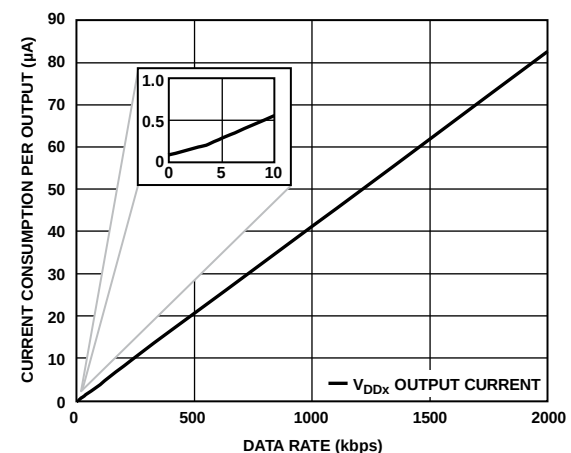
Figure 16. Current Consumption per Output vs. Data Rate for 2.5 V, \text{EN}_x = \text{High Operation}
