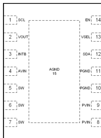
(Top View) 14-Pin 0.50 mm pitch DFN
