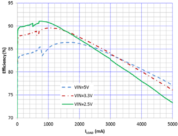
Figure 10. Efficiency vs I_{LOAD} and V_{IN} , V_{OUT} = 1.150 V
