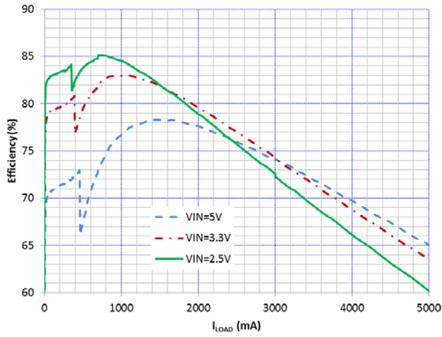
Figure 12. Efficiency vs I_{LOAD} and V_{IN} , V_{OUT} = 0.600 V
