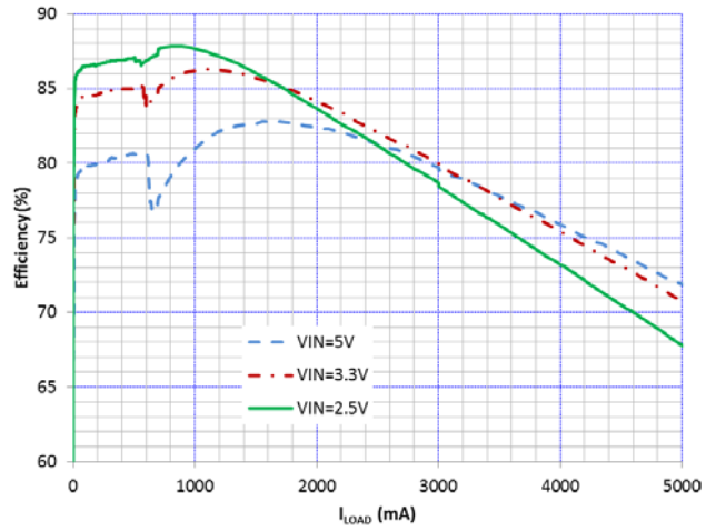
Figure 13. Efficiency vs I_{LOAD} and Temperature, V_{OUT} = 0.875 V , HEI201612A-R24M Inductor
