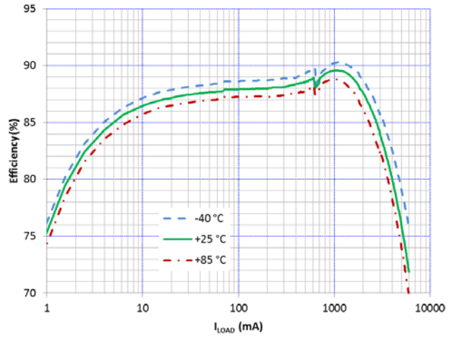
Figure 11. Efficiency vs I_{LOAD} and Temperature, V_{OUT} = 1.150 V
