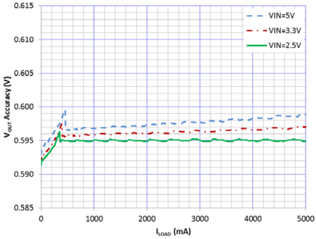
Figure 18. V_{OUT} Accuracy vs I_{LOAD} and V_{IN} , V_{OUT} = 0.600 V
