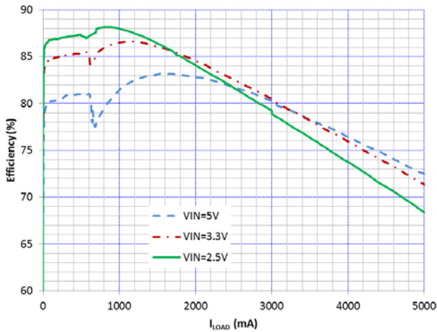
Figure 14. Efficiency vs I_{LOAD} and Temperature, V_{OUT} = 0.906 V , HEI201612A-R24M Inductor
