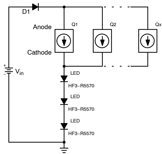
Figure 8. Typical Application Circuit (60 mA each LED String)
