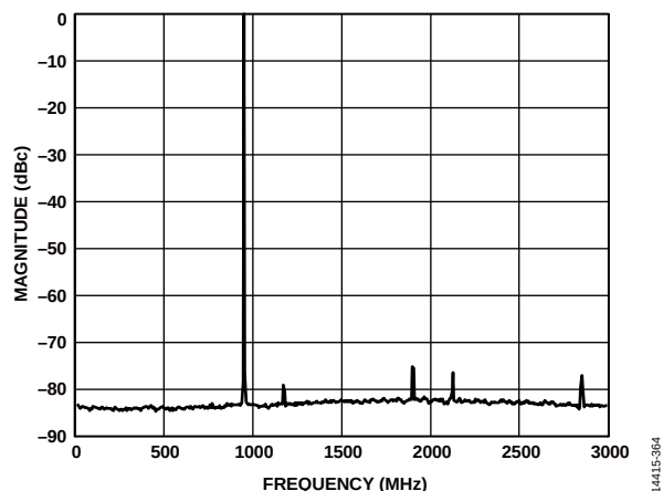
Figure 68. Single Carrier at 950 MHz Output (Shuffle On)
