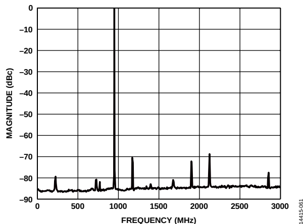
Figure 65. Single Carrier at 950 MHz Output
