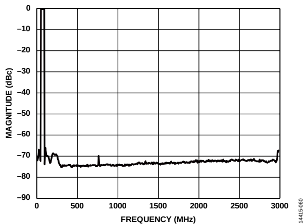
Figure 61. Eight Carriers at 70 MHz Output
