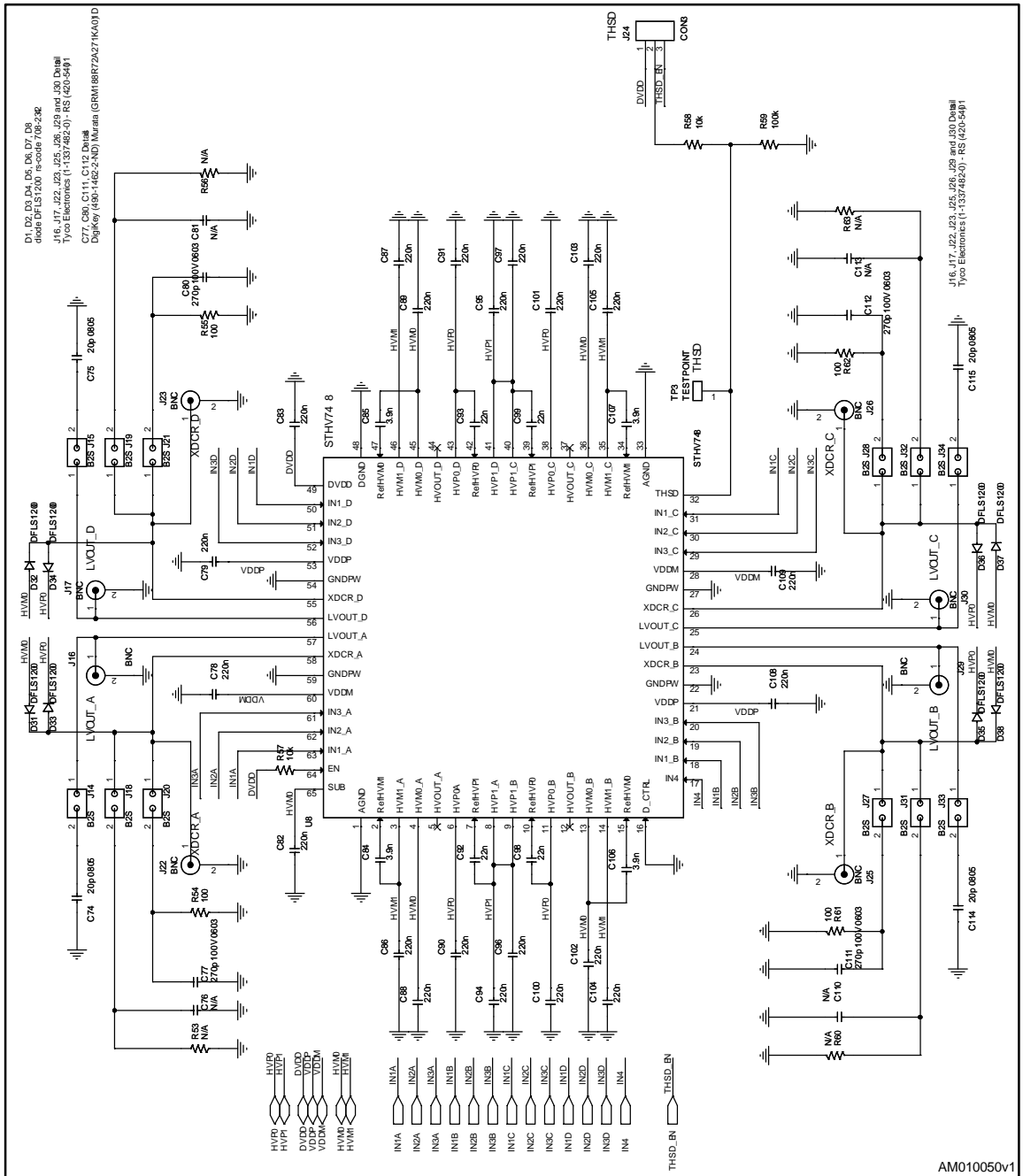
Figure 8: STEVAL-IME003V1 configuration of the STHV748
