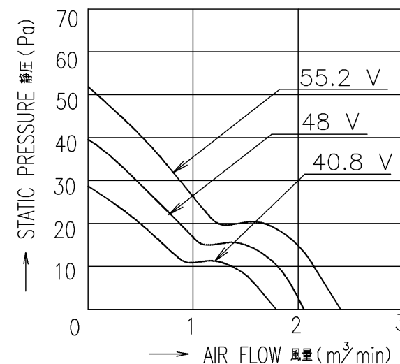
PERFORMANCE CURVES
