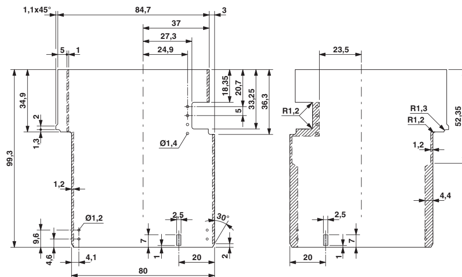
Dimensional drawing
