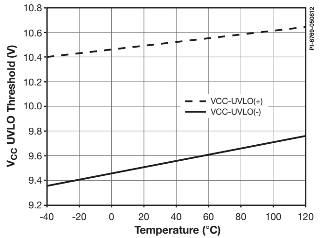
Figure 42. Typical V_{CC UVLO} vs. Temperature.
