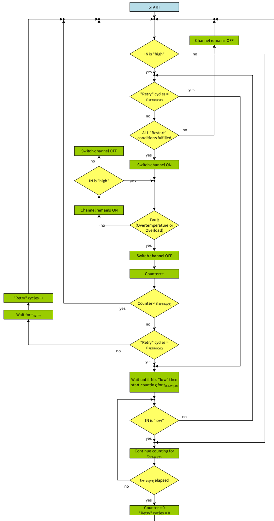
Figure 29 Retry Strategy Flowchart
