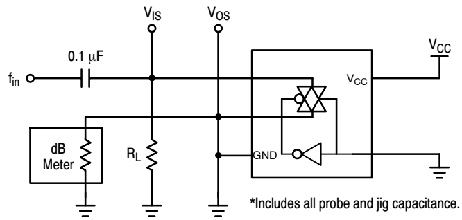
Figure 9. Off-Channel Feedthrough Isolation Test Set-Up
