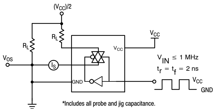
Figure 11. Feedthrough Noise, ON/OFF Control to Analog Out, Test Set-Up
