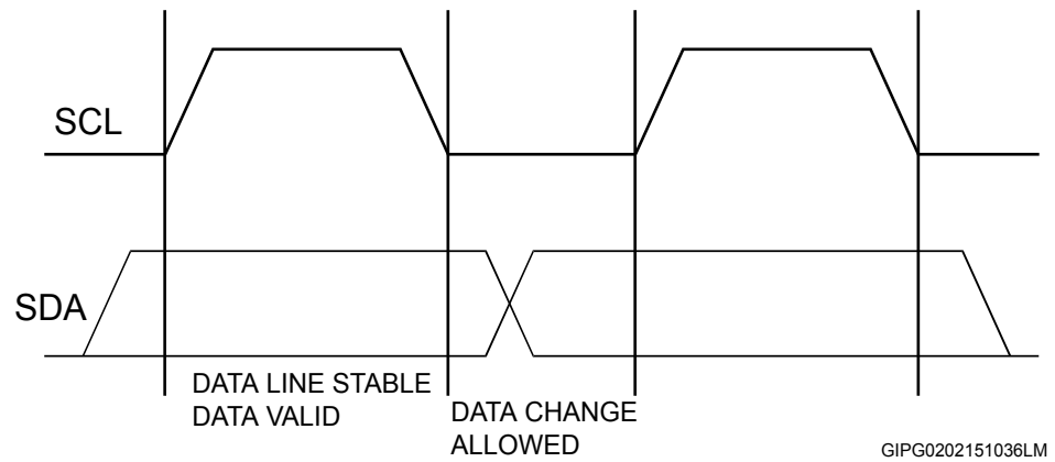
Figure 9. Timing diagram of I 2 C bus
