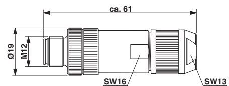
Plug, M12 x 1, straight, shielded
