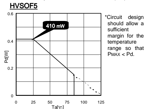
Fig.27 HVSO5 Power Dissipation vs Heat Reduction (Example)
