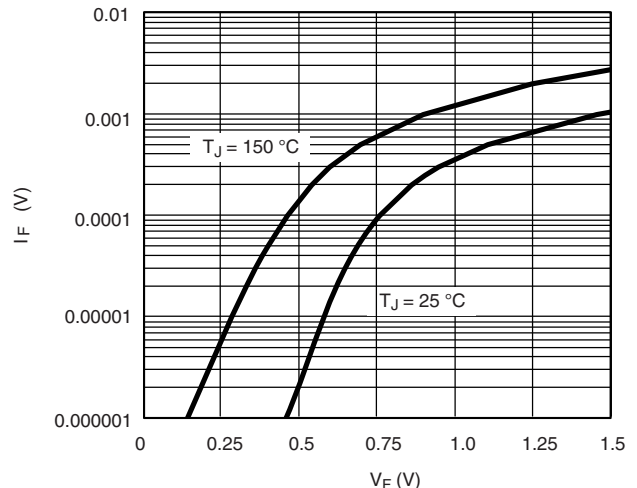
Sense Diode Forward Voltage
