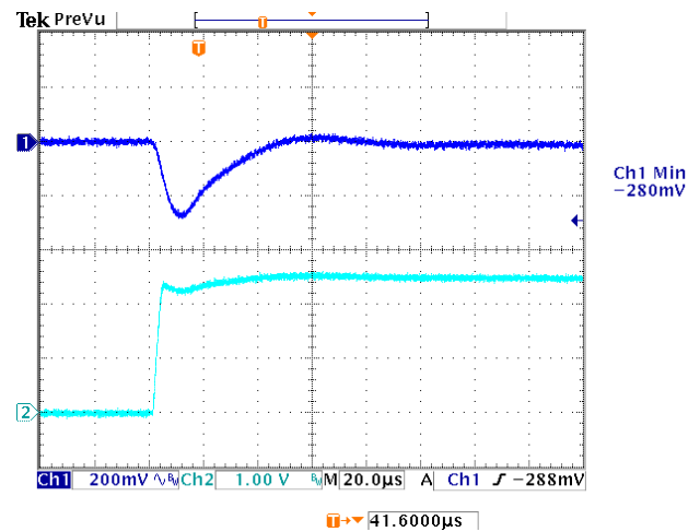
Figure 24: Typical Transient Response to Step Load Change at 2.5A/\mu S from 50% to 100% of I_o , max at 3.3V_{in} , 2.5V_{out} ( C_{out} = 1\mu F ceramic, 10\mu F Tantalum)
