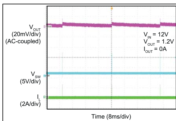
FIGURE 2-47: MIC2125 Switching Waveform, I_{OUT} = 0A .
