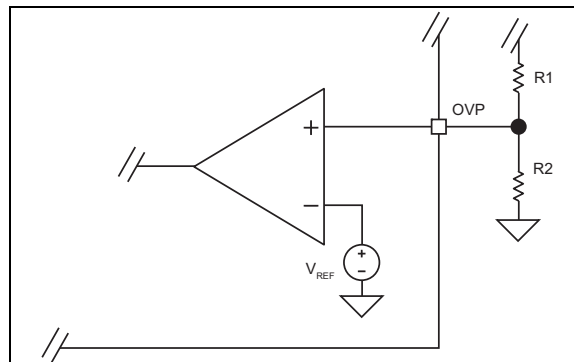
FIGURE 5-4: OVP Voltage-Divider Configuration.
