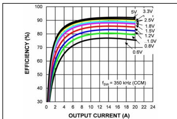
FIGURE 2-31: Efficiency ( V_{IN} = 18V ) vs. Output Current (MIC2126).
