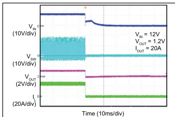
FIGURE 2-33: V_{IN} Soft Turn-Off.
