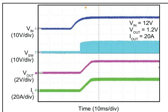
FIGURE 2-32: V_{IN} Soft Turn-On.
