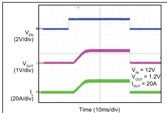
FIGURE 2-35: Enable Turn-On/Turn-Off.
