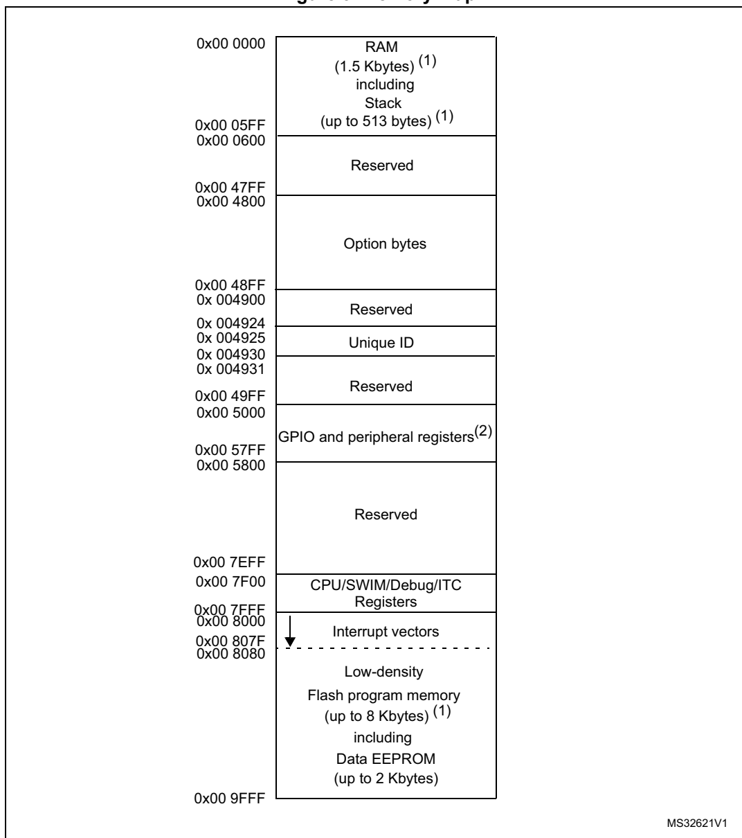
Figure 3. Memory map
