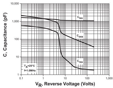
Capacitance
