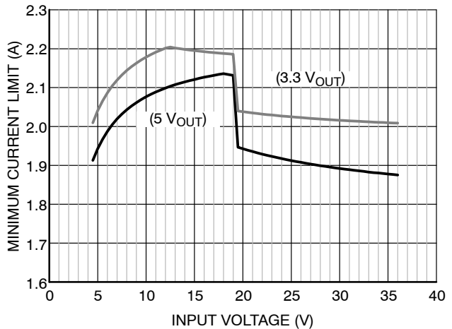
Figure 28. NCV890201 Load Current Capability with 4.7 \mu\text{H} Inductor
