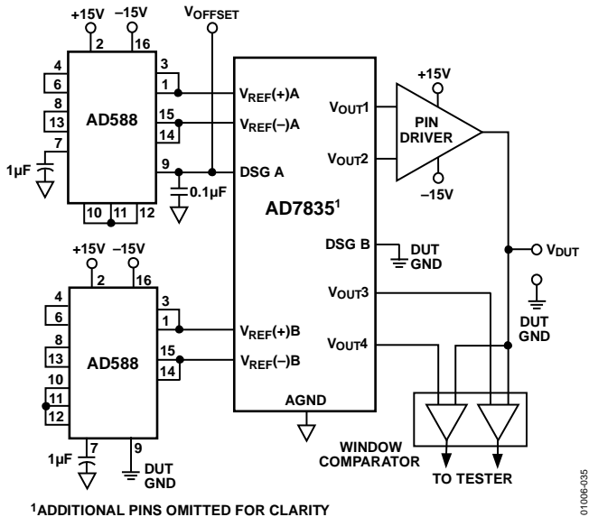
1ADDITIONAL PINS OMITTED FOR CLARITY Figure 35. ATE Application
