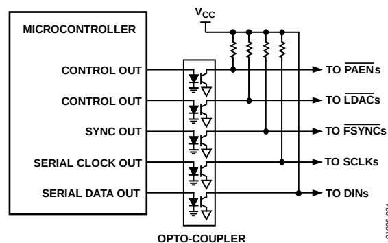
Figure 34. Opto-Isolated Interface
