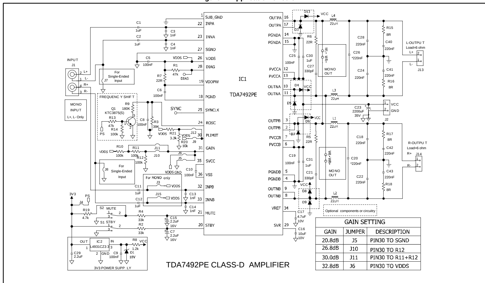
Figure 7: Application circuit
