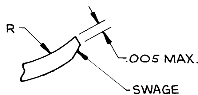
DETAIL A SCALE 20:1
