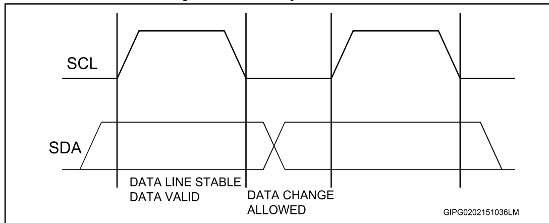
Figure 5: Timing diagram of I 2 C bus
