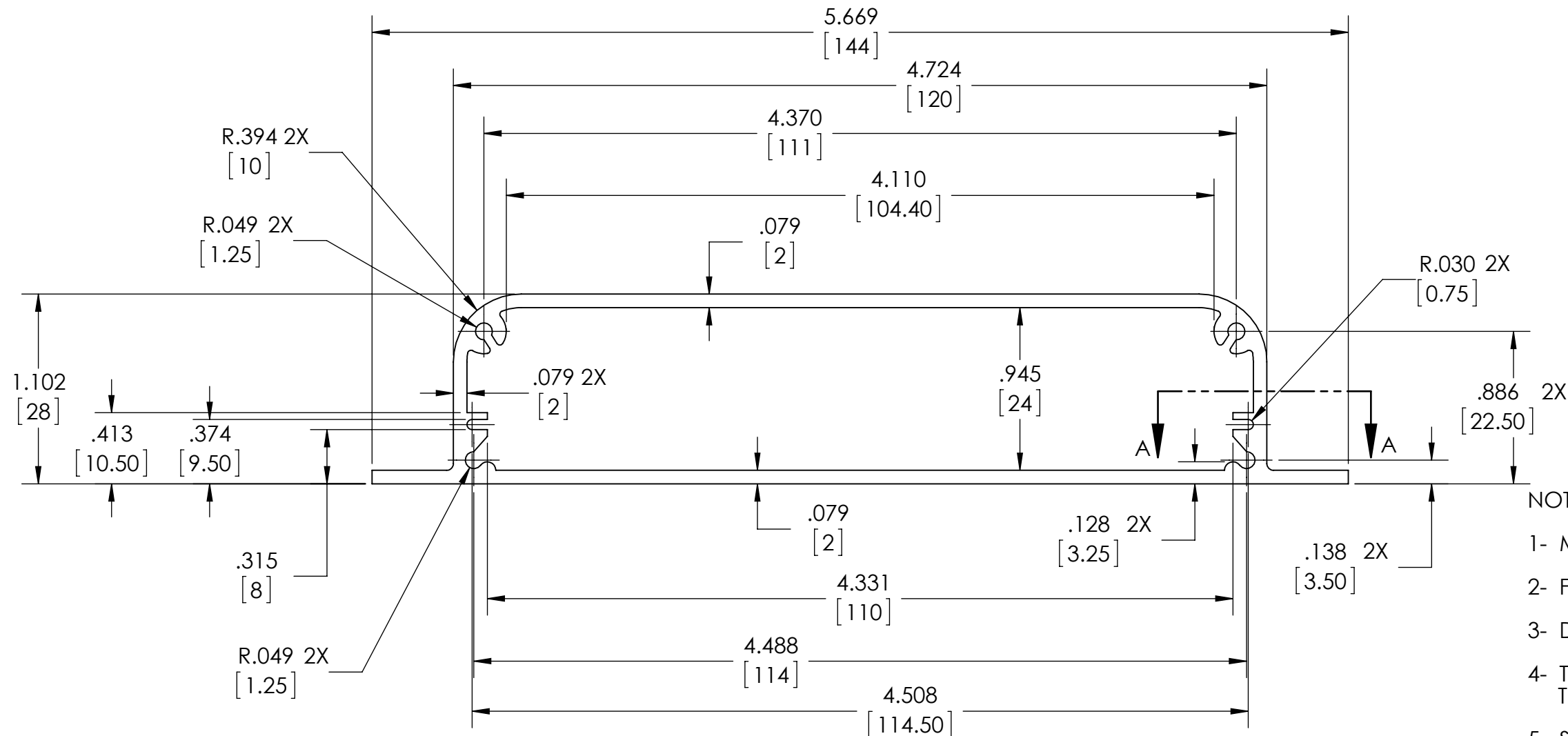
EXTRUSION PROFILE
