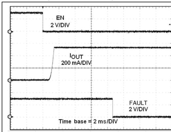
Figure 38. OC protection at V_{OUT} = 3.0\text{ V} (STMPS2161/2171)
