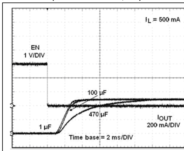
Figure 34. Current output turn-on delay time (STMPS2161/2171, 3 V)
