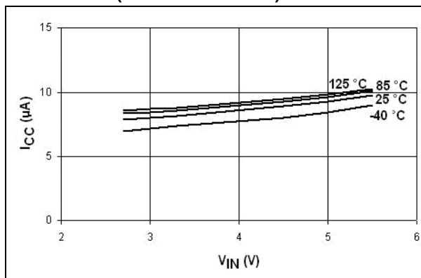
Figure 19. I_{CC} vs. V_{IN} (disabled) (STMP2141/2151)
