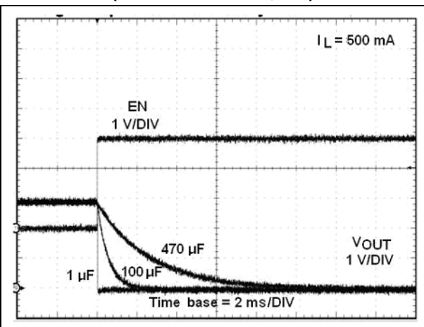
Figure 33. Voltage output turn-off delay time (STMPS2161/2171, 3 V)
