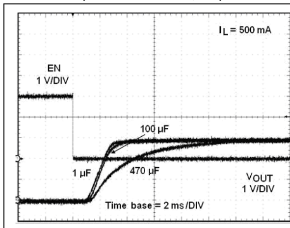
Figure 32. Voltage output turn-on delay time (STMPS2161/2171, 3 V)
