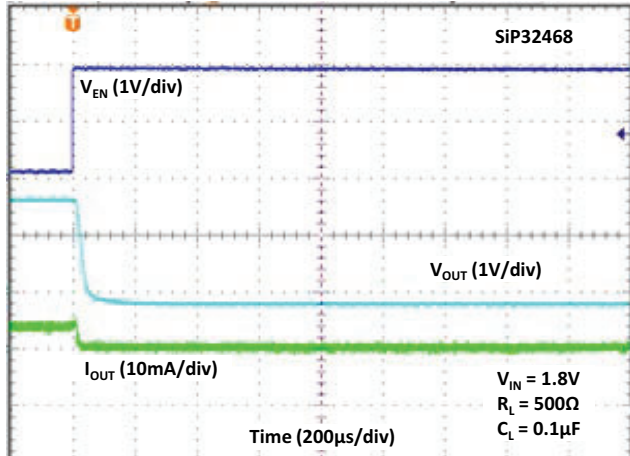
Fig. 33 - Turn-off Time
