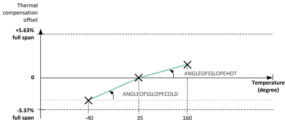
Figure 10 - Input range from -40Deg.C up to 160 Deg.C
