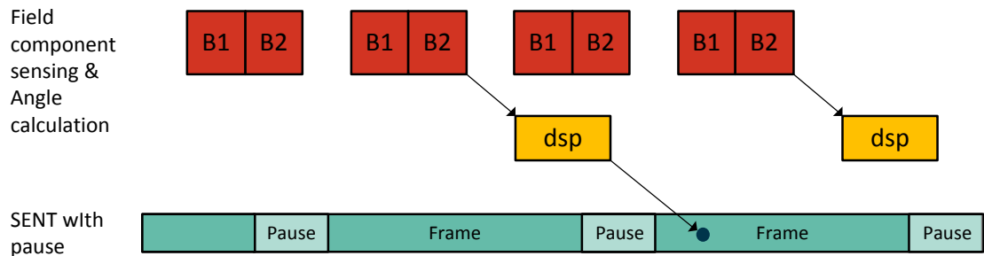
Figure 4 - Latency - Case FILTER = 0 (not recommended)
