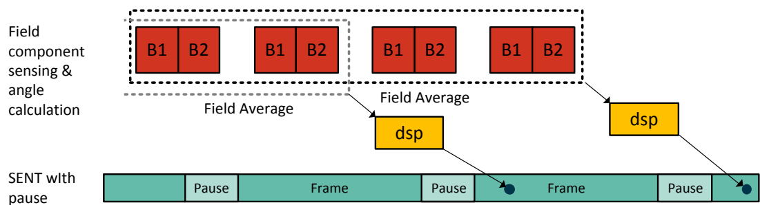
Figure 5 - Latency - Case FILTER = 2
