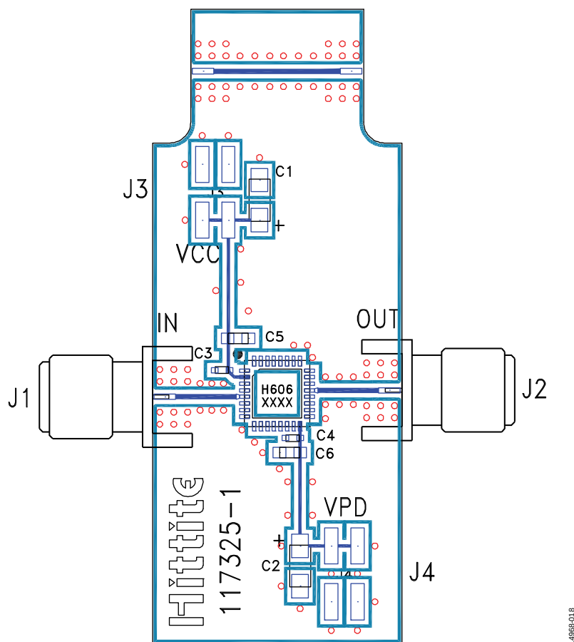
Figure 17. Evaluation PCB
