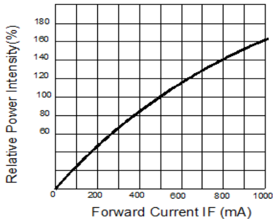
Relative Radiant Flux vs. Forward Current (Ta=25°C)
