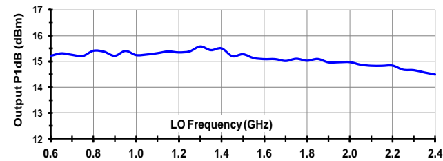
1dB Compression
