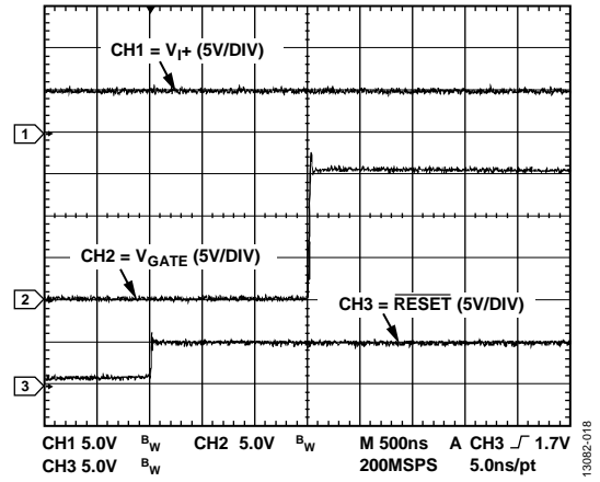
Figure 18. Example RESET to Output Valid
