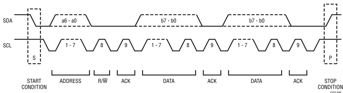
Figure 6. Data Transfer Over I²C or SMBus
