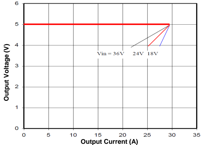
Figure 10. Output Characteristics
