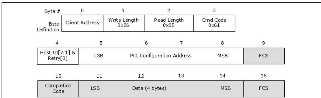
Figure 2-45. RdPCIDebug()
