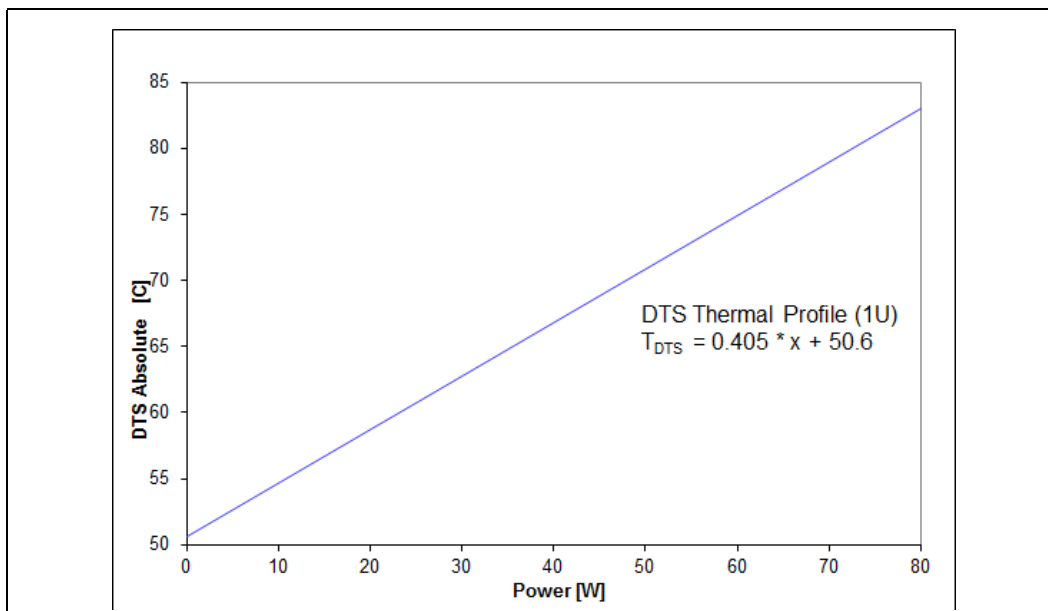
Figure 5-26. DTS: 4-Core 80W Thermal Profile 1U
