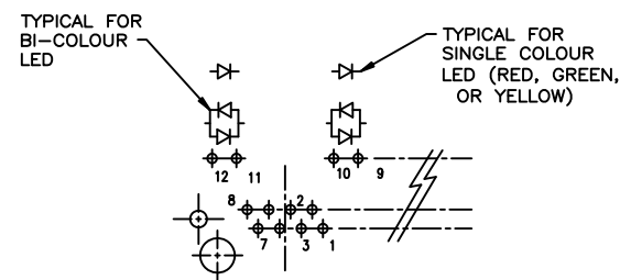
LED SCHEMATIC
